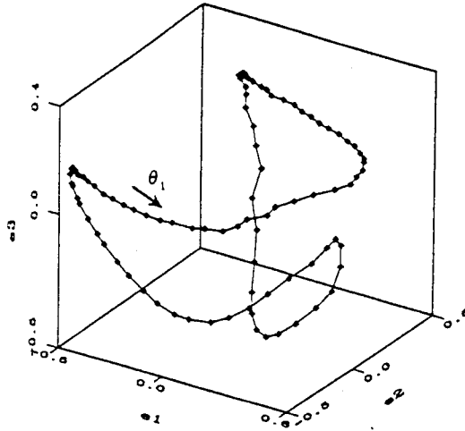
Figure 2: Parametric eigenspace representation of the object shown in Fig.1. Only the three most prominent dimensions of the eigenspace are displayed here. The points shown correspond to projections of the learning samples. Here, illumination is constant and therefore we obtain a curve with a single parameter (rotation) rather than a surface.
